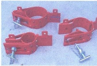
4, 6 & 8 inch elevators
